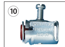
10 Size: 1/2"; P/N E00-005-002 Type: Speed Lock Style, Snap-in Material: Steel Insulated: Yes
