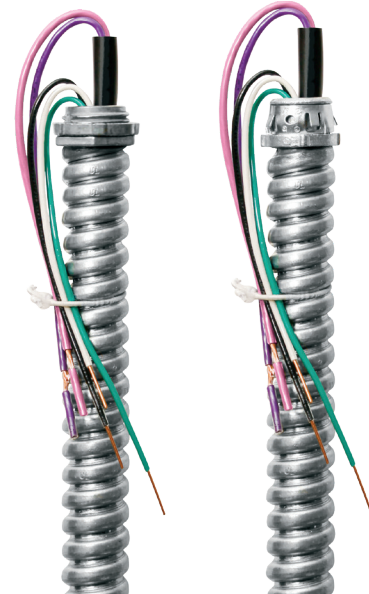
120-Volt, Die Cast Screw-In Connector
