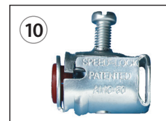
10 Size: 1/2": P/N E00-005-002 Type: Speed Lock Style, Snap-in Material: Steel Insulated: Yes
