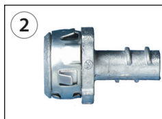
2 Size: 1/2": P/N E00-005-000 Type: Screw-in/Snap-in Material: Die Cast Insulated: Yes or No (circle one)
