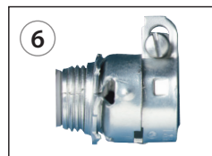
6 Size: 1/2": P/N E00-042-002 Type: Set Screw, Squeeze Material: Steel Insulated: 3/8": No 1/2": Yes
