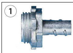
1 Size: 1/2": P/N E00-026-000 Type: Screw-in (lock-nut) Material: Die Cast Insulated: Yes or No (circle one)
