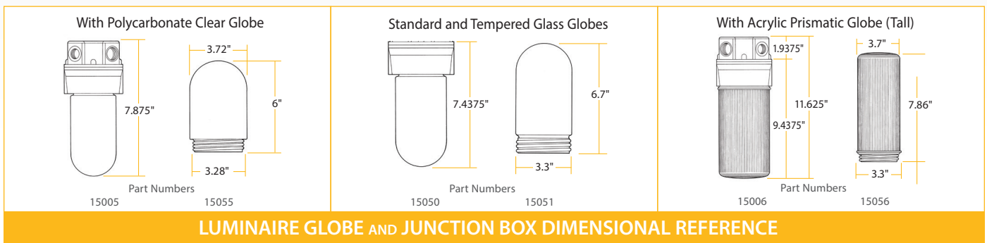
CEILING MOUNT LUMINAIRE
