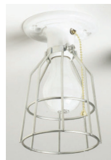
Lamp Holder (P/N: 16512) shown with Metal Safety Cage (P/N: 16501)
