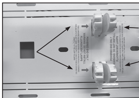
Figure 7: Place, rotate, and "fully" seat the Type "B" Single-End Powered T8 LED Tubes into the lamp holders.
