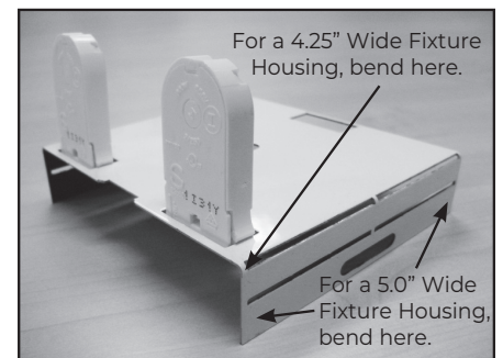
Figure 3: RetroFit Socket Plate for Installation on a 4.25" wide Luminaire Housing.
