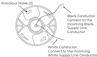
Figure 1. Bottom view of Keyless LED Luminaire
