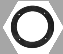
Neoprene Gasket P/N E05-003-002
