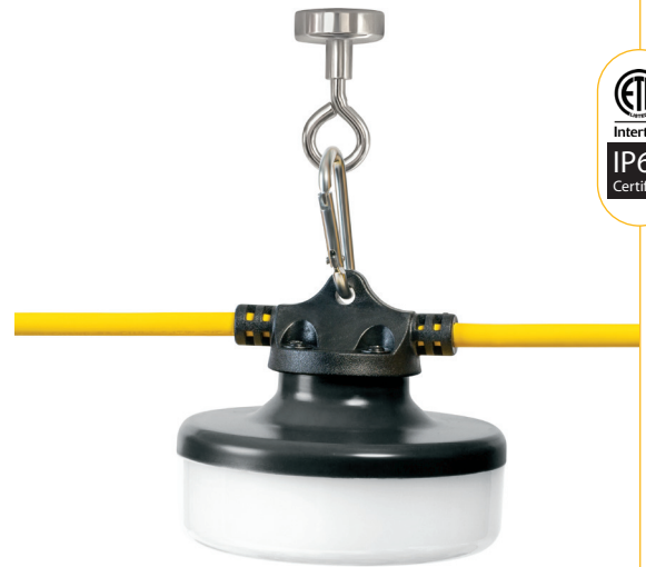
LED CordLights (Standard Lumen Output, 1,500 Lumens per Module) Shown with Magnetic Suspension Hanger Part Numbers: 16140 and 16145; Magnetic Suspension Hanger: CORDLIGHT-MH
