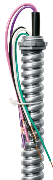
Illumination Control Health Care Fixture Whip Shown with Standard Screw-In Lock Nut Connector
